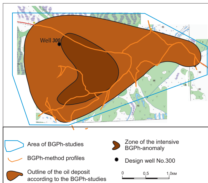
Fig. 4. Results of the BGPh-studies at the Tlanchi-Tamasky section. Note: Well No. 300 was drilled in the spring of 2014, the oil deposit in C1bb was penetrated. The total capacity of oil-saturated reservoirs is 10 m
